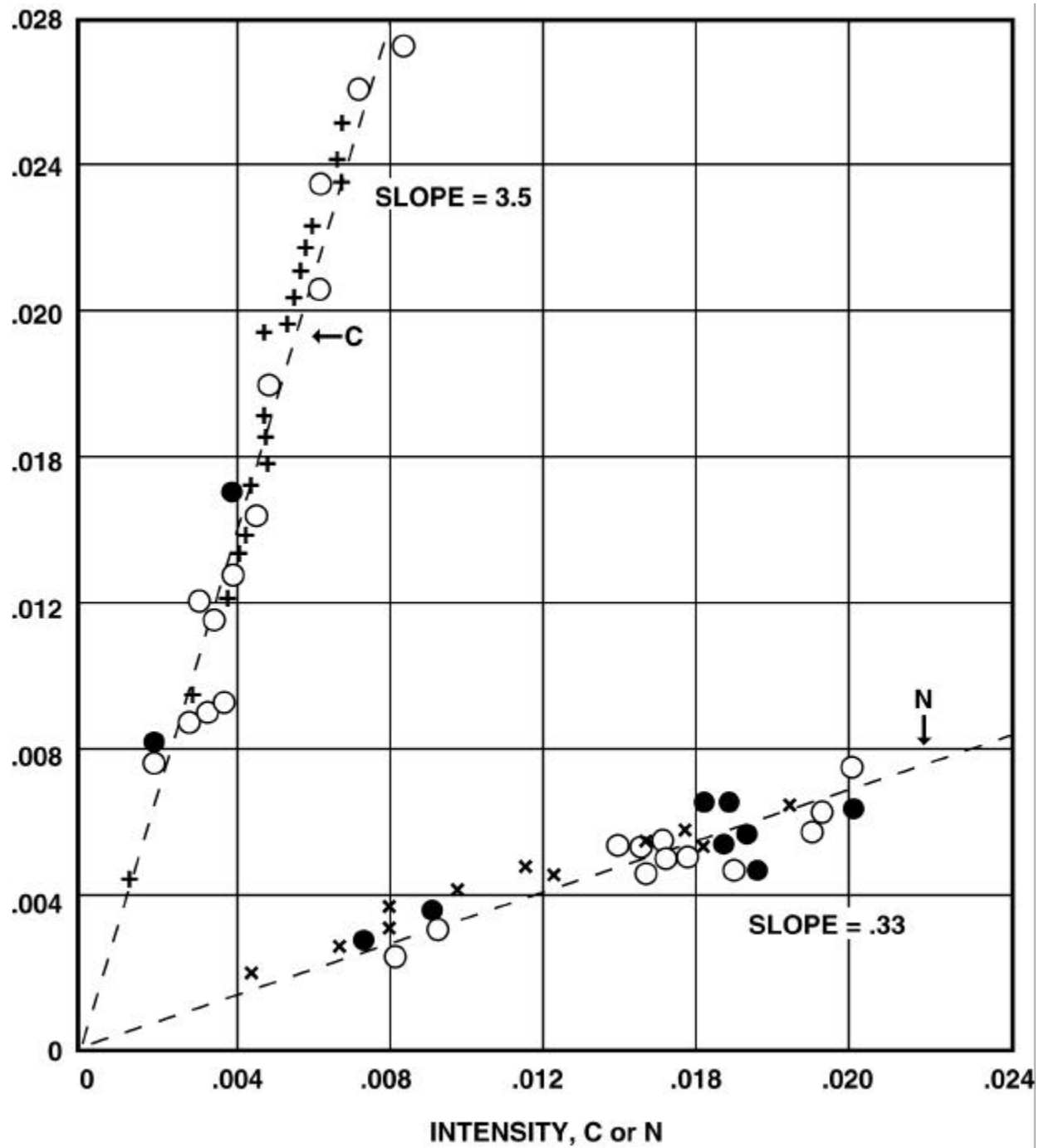
Correlation of A, N, and C strips as checked on an Almen Gage No. 2
