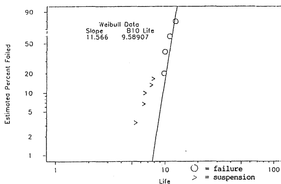
Figure 5. Weibull probability plot of gear life at 3.2L SHO loads with lowest cost shotpeen.
