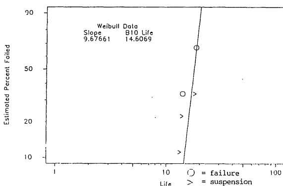
Figure 2. Weibull probability plot of gear life potential at 3.8L loads using shotpeen.
