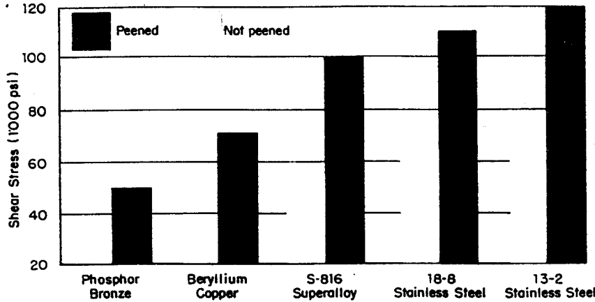
Fig. 1--Safe fatigue-life ranges for coil springs of various materials, indicating increased life available with shot peening
