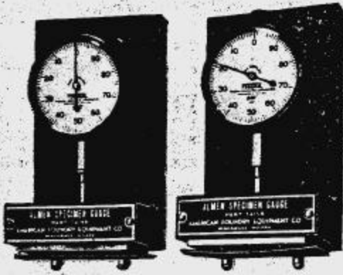
Fig. A--Almen paring-intensity gages checking curvature of unpeened (left) and peened (right) strips.
