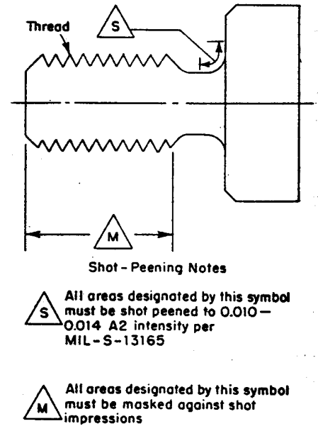
Fig. 18--Drawing of typical part, with peening notes and specifications
