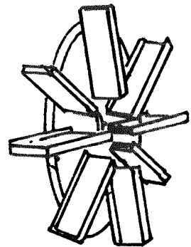
FIG. 7 Single Sided Blast Wheel.
