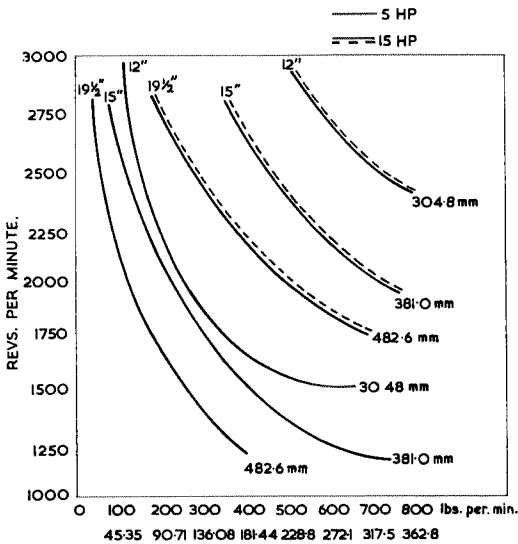
WHEEL SPEED vs. ABRASIVE FLOW.
