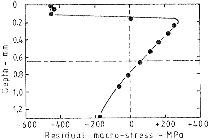
Fig.2 Residual Macro-stress Profile in Peen-formed Strip
