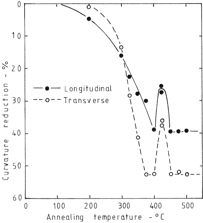
Fig.1 Curvature relief on Isochronal Annealing
