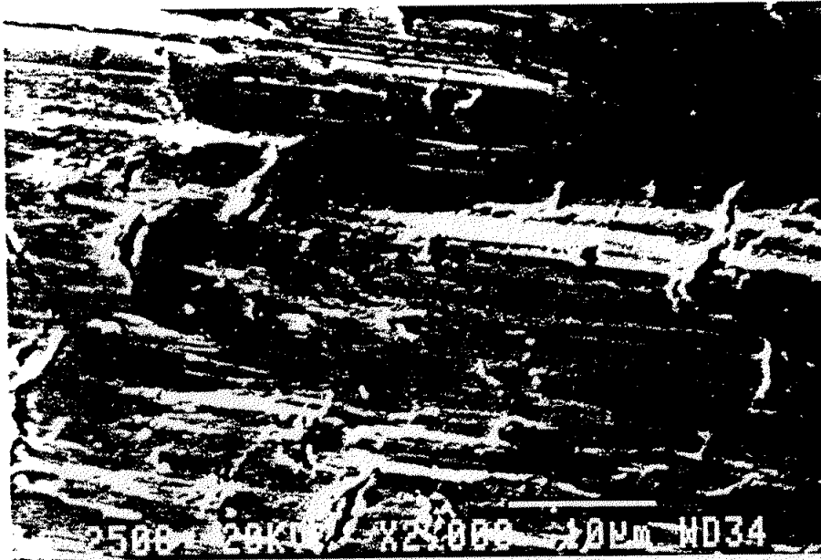
photo4: ductile area of the fracture surface 0.1mm beneath the surface
