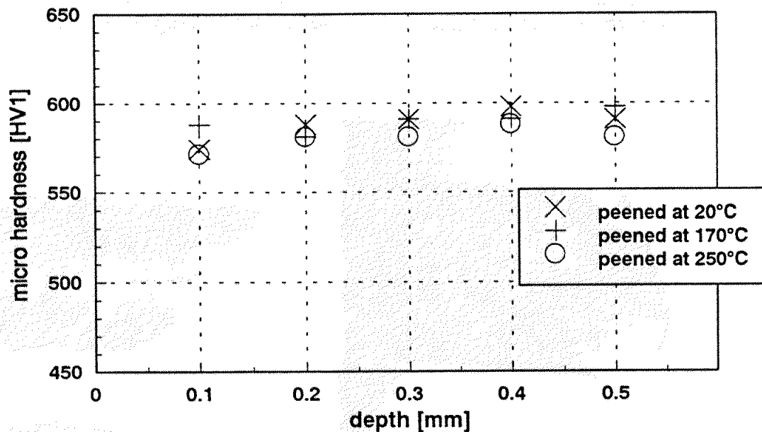
Figure 2: Vickers hardness of the surface layer
