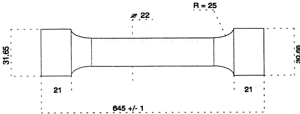
Figure 1: specimen configuration in [mm]
