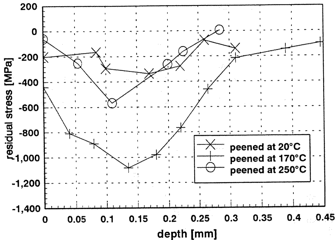
Figure 5: residual stress profiles after fatigue testing
