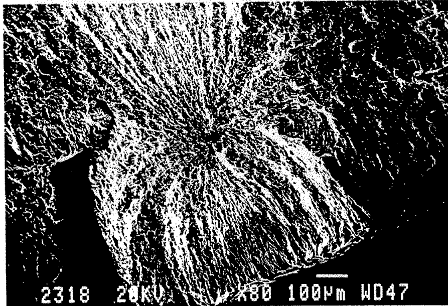
photo2: crack initiation from an inclusion with a radial line pattern
