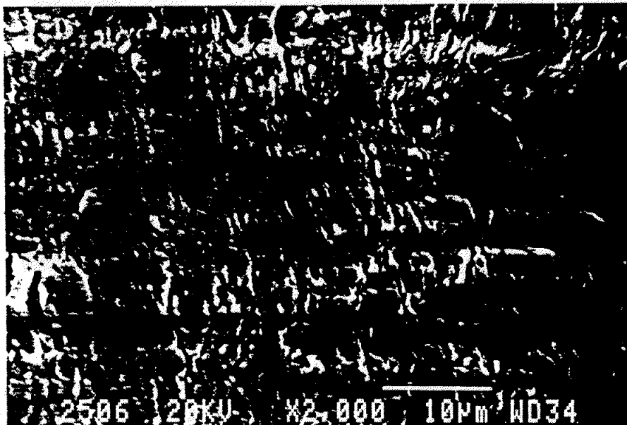
photo3: ductile area of the fracture surface 1mm beneath the surface
