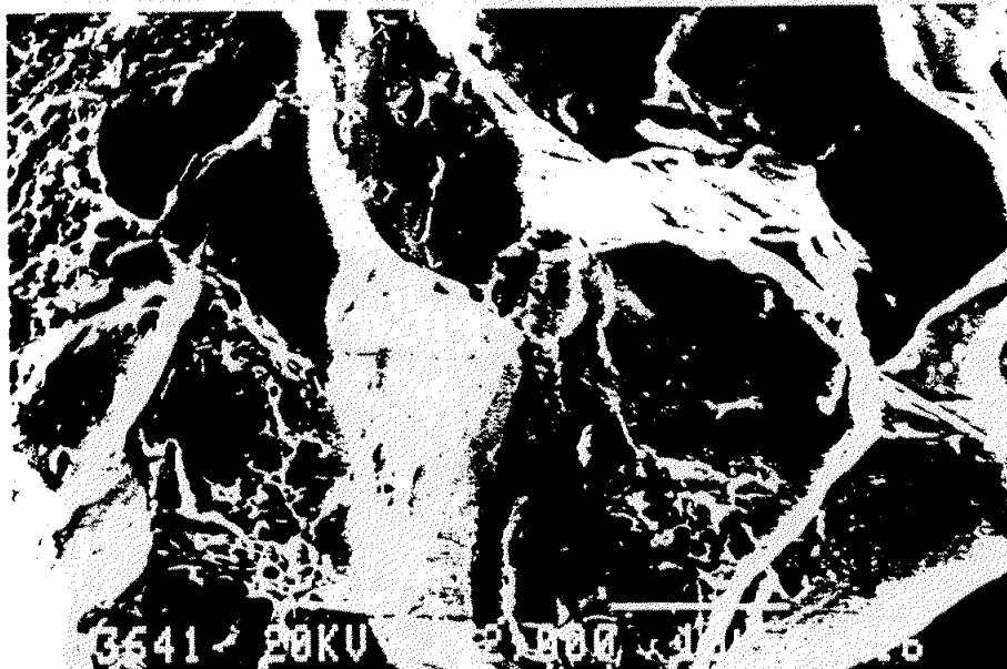
photo5: fragile area of the fracture surface
