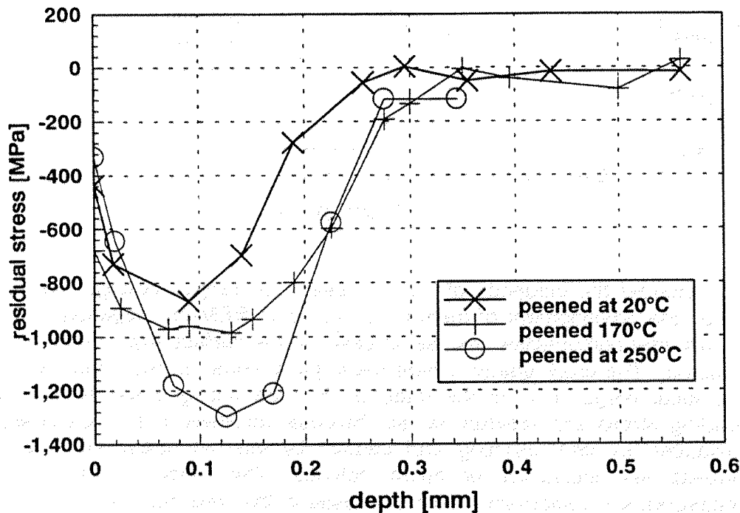
Figure 4: residual stress curves before fatigue testing
