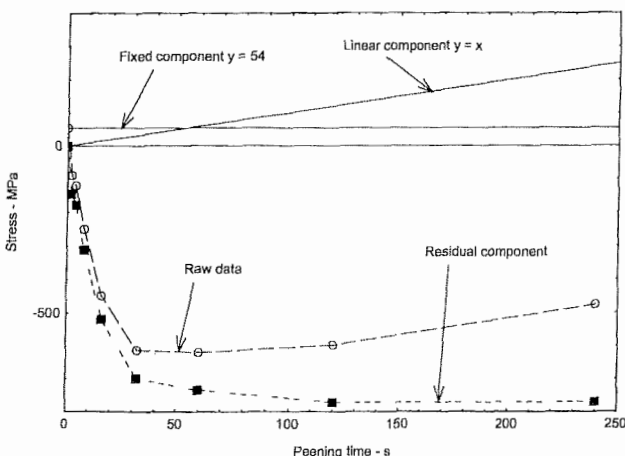
Fig.6 Components of raw stress/peening time data.
