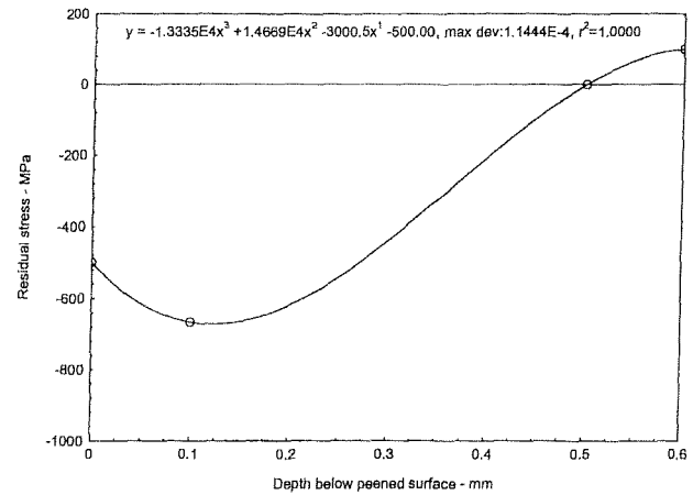
Fig.15 Model of residual stress/depth profile.
