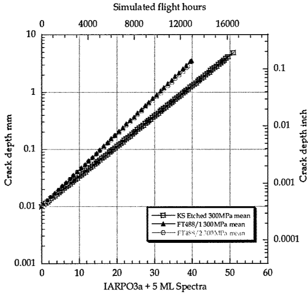
Figure 42. The mean crack growth slopes for the KS plate (Etched) and the two sets of specimens from the FT488/1 and FT488/2 tests, for the 300MPa stress level.
