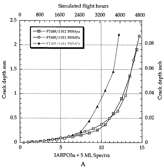
Figure 18 The result of the quantitative fractographic examination of cracks in the FT488/1 specimens loaded to a peak stress of 390MPa.
