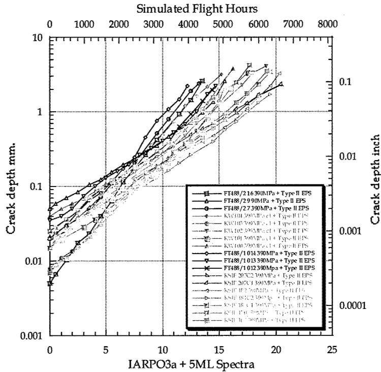
Figure 40. The plots of the two Y488 bulkhead sets of specimens compared to the KS and KW plate data for the 390MPa stress level. Note that the KW data appears to be more like the FT488/1 and 2 data.
