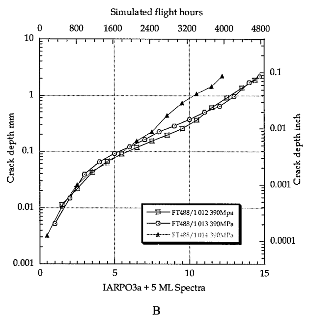
Figure 18 The result of the quantitative fractographic examination of cracks in the FT488/1 specimens loaded to a peak stress of 390MPa.
