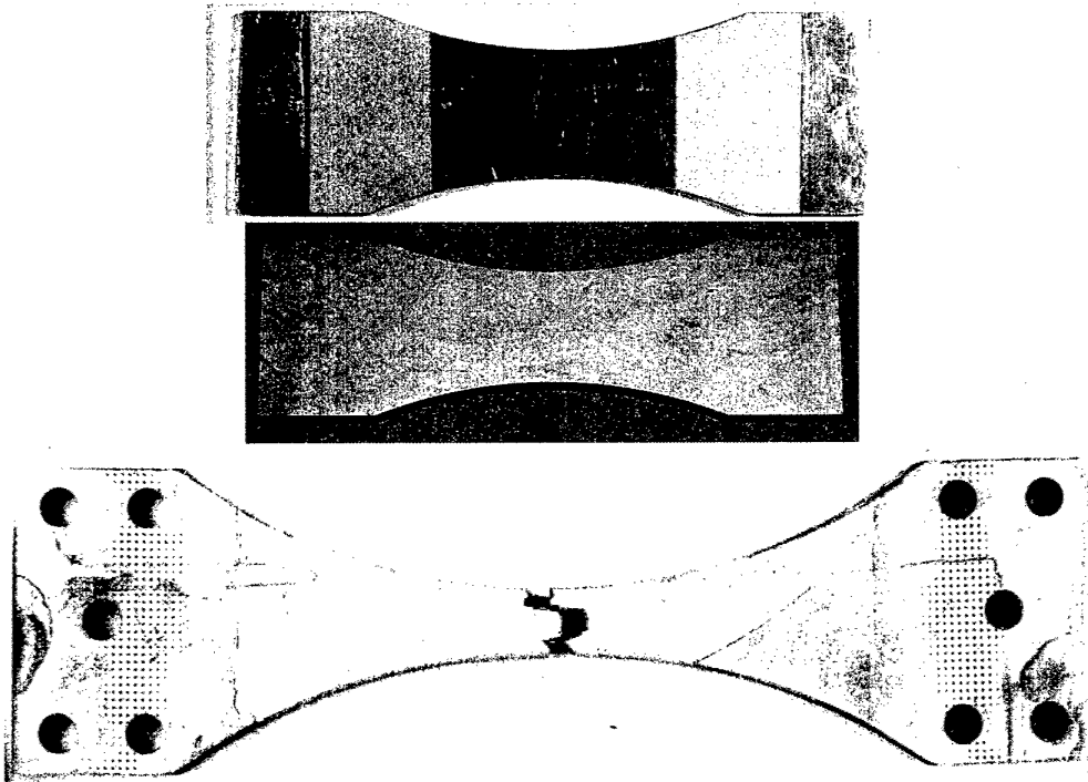
Figure 2 Pictures of the three types of specimens - the first shows a specimen cut from the FT488/1 bulkhead, peened in the grip areas and on the cut edges, and the second picture is of an etched specimen cut from the KW plate. The third picture is of one of the KS specimens (after failure), which were used for comparison purposes in this report.
