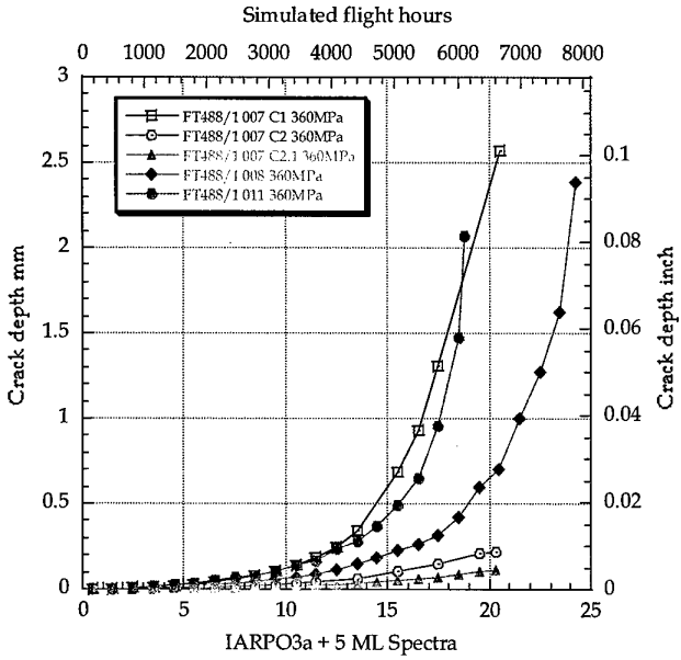
Figure 17 The result of the quantitative fractographic examination of cracks in the FT488/1 specimens loaded to a peak stress of 360MPa.
