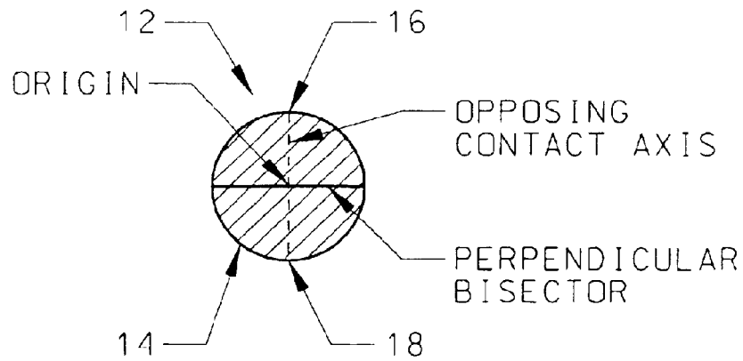
Section B-B of Figure 1A
