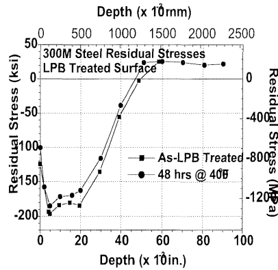
Figure 7 – LPB subsurface residual stress distributions.
