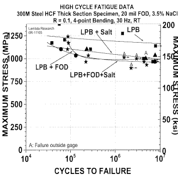
Figure 10 - Fatigue results for LPB
