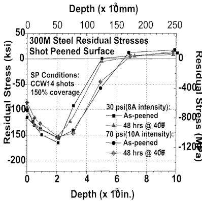
Figure 6 – SP subsurface residual stress distributions.
