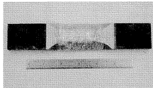
FIGURE 4 - A thick section specimen with salt solution soaked tissue wrapped around the gage section.
