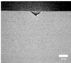
FIGURE 3 - Cross-section of 0.5 mm deep EDM notch to simulate FOD.
