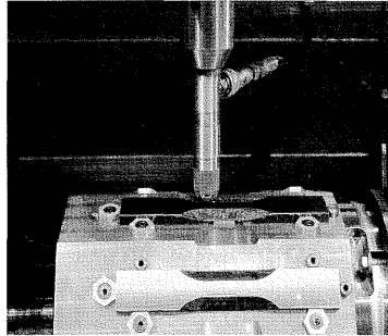
Figure 2 - A set of 8 thick section specimens being LPB processed in a 4-axis CNC milling machine.
