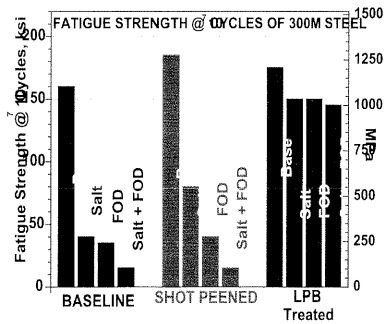
Figure 11 - Summary of fatigue results.
