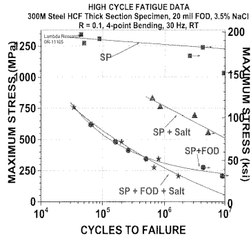
Figure 9 - Fatigue results for SP.
