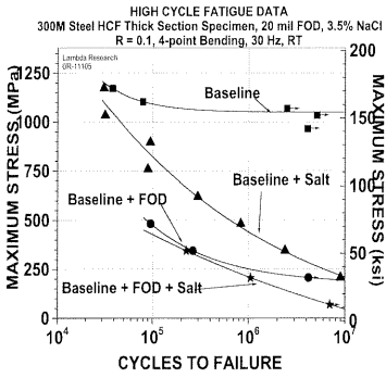
Figure 8 - Baseline fatigue results.
