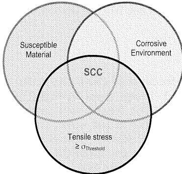
Figure 1 - SCC susceptibility diagram
