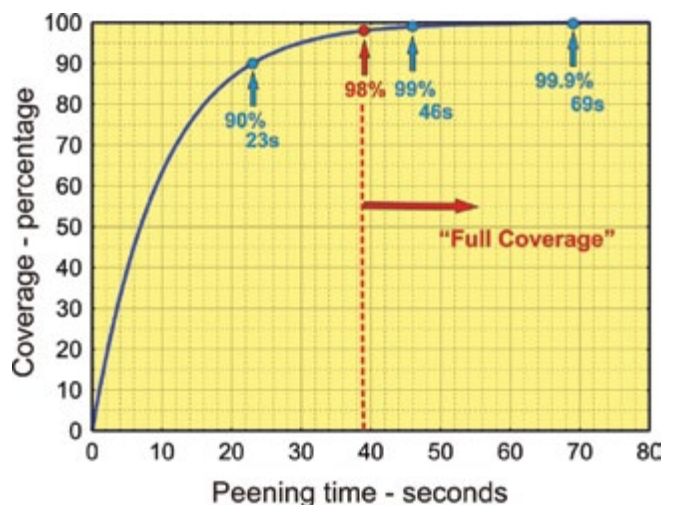
Fig.5 Coverage curve when Coverage Factor equals 0.1s -1 .
