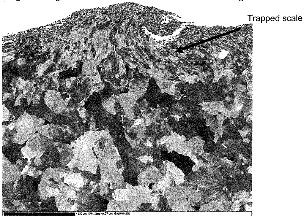
Fig 4 EBSD image of the first 300 µm in a shot-blasted connecting rod. Scale has been trapped in a 50 µm fold during the shot-blasting.
