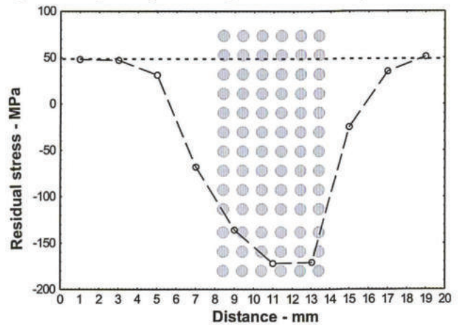
Fig.8 Variation of surface residual stress with distance across peened mild steel plate.
