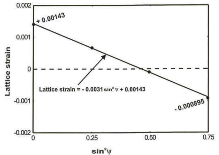
Fig.4 Linear relationship between lattice strain and \sin^2 \psi .
