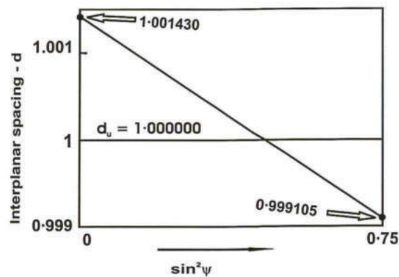
Fig.5 Data from fig.4 plotted in terms of interplanar spacings.
