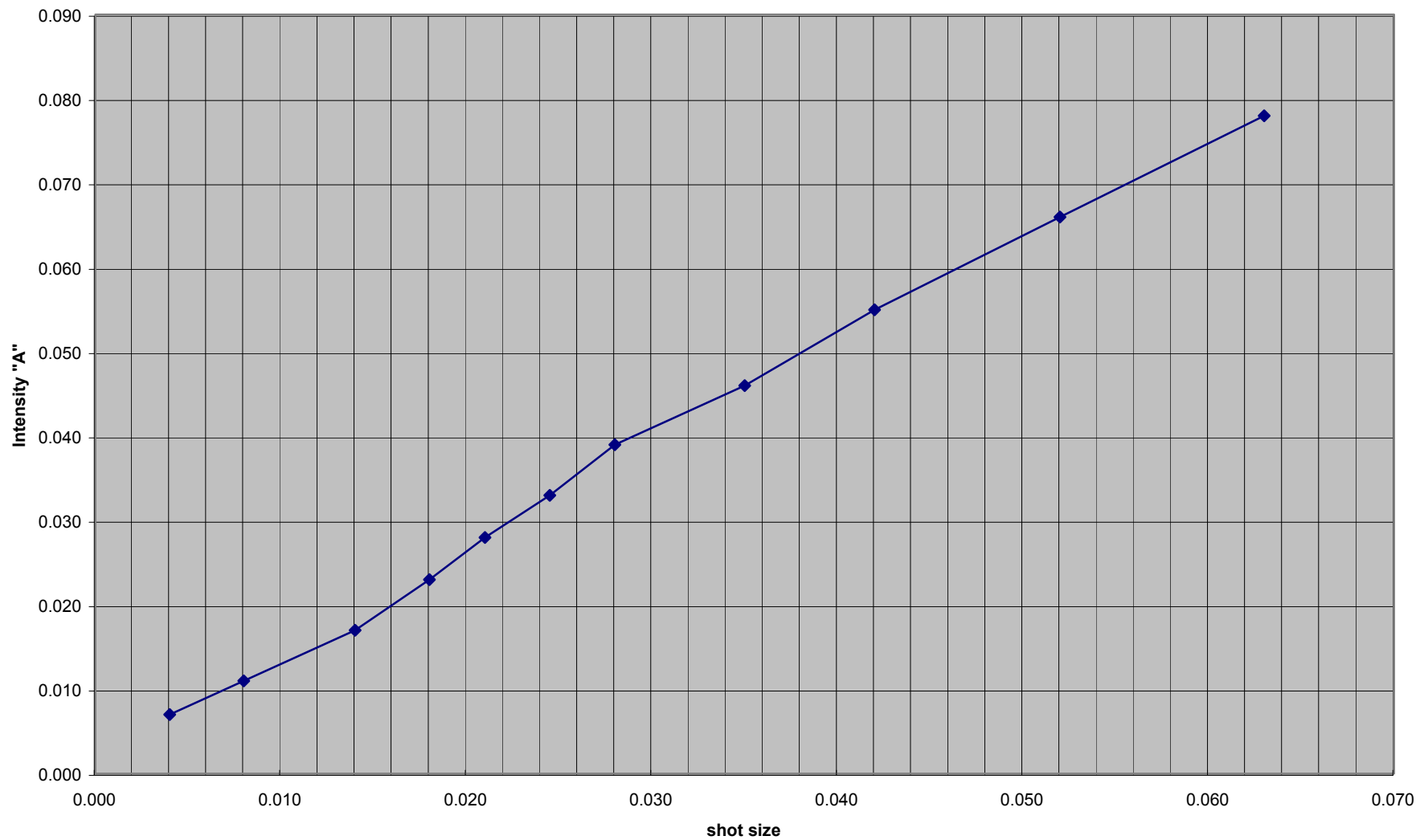
Intensity as function of shot size 245 F/S 19.5" wheel at 2250 RPM courtesy of Wheelabrator Corporation
